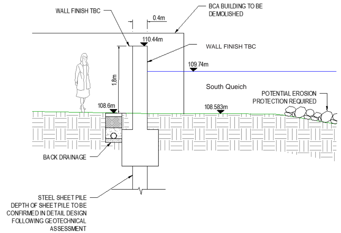
Location 4: Typical Flood Wall Detail at BCA Site*
