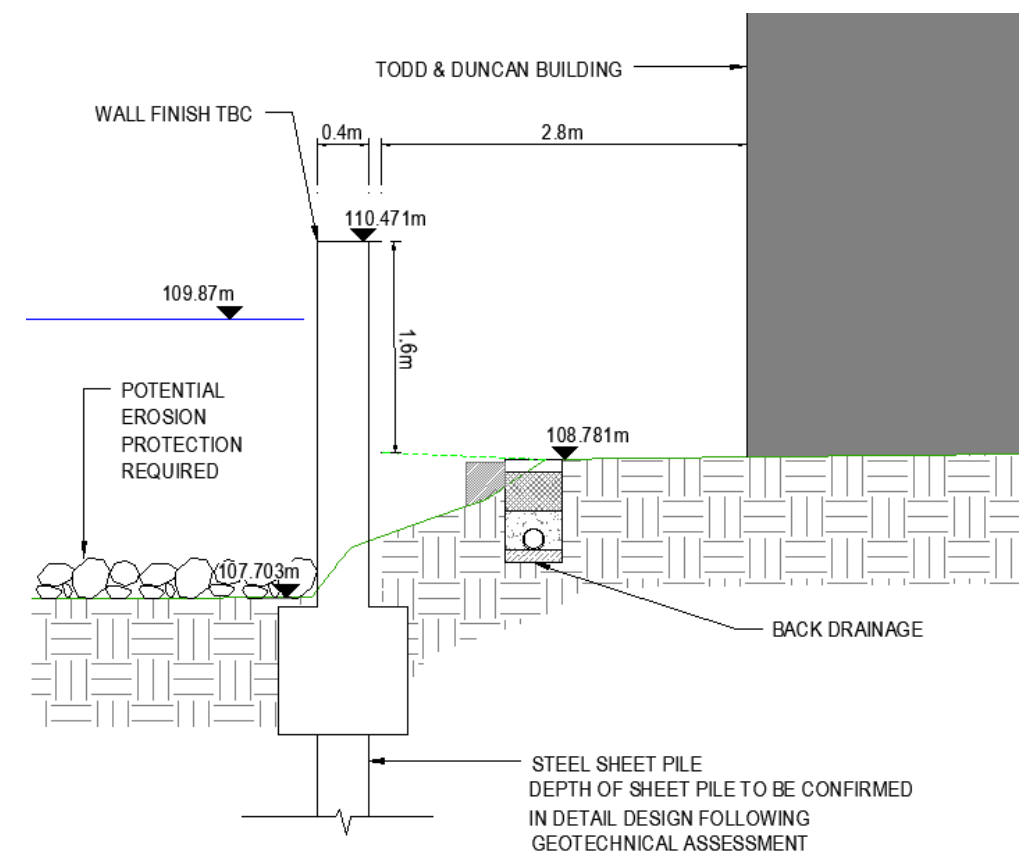
Location 5: Typical Flood Wall Detail at Todd & Duncan*
