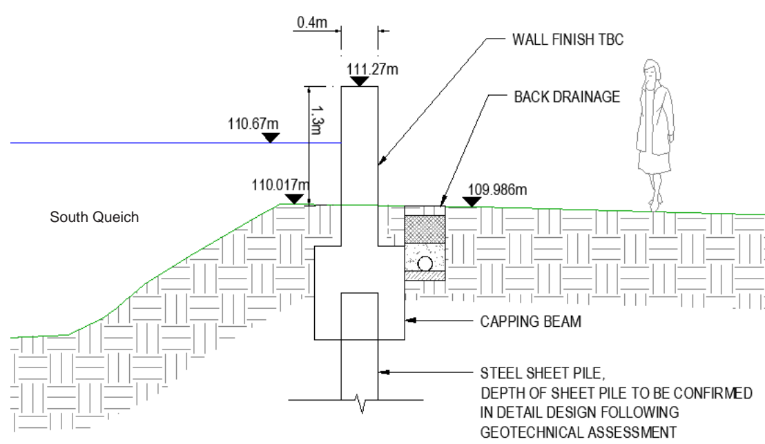
Location 3: Typical Flood Wall Detail at Queich Place*
