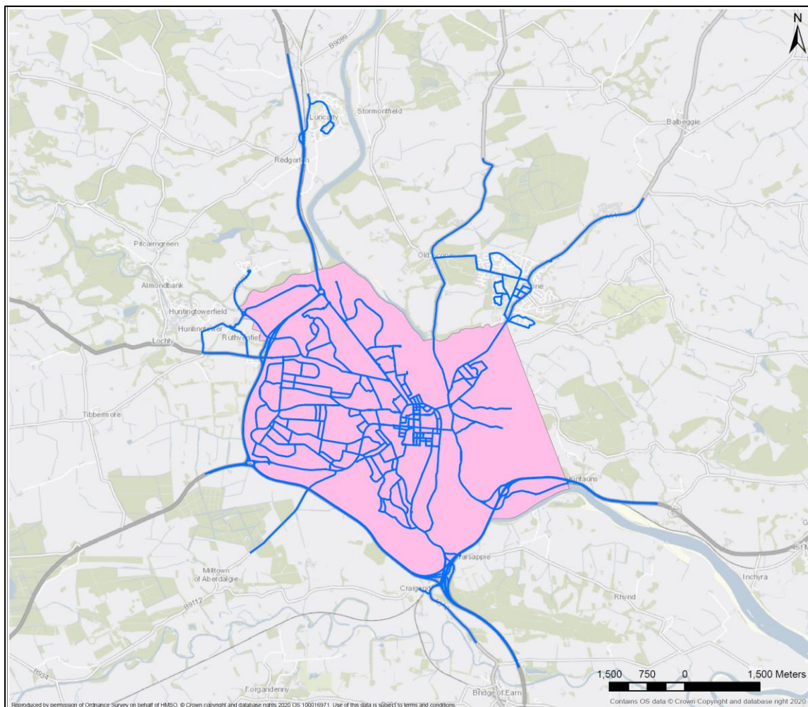
Figure 6.1: Air quality Model Domain
