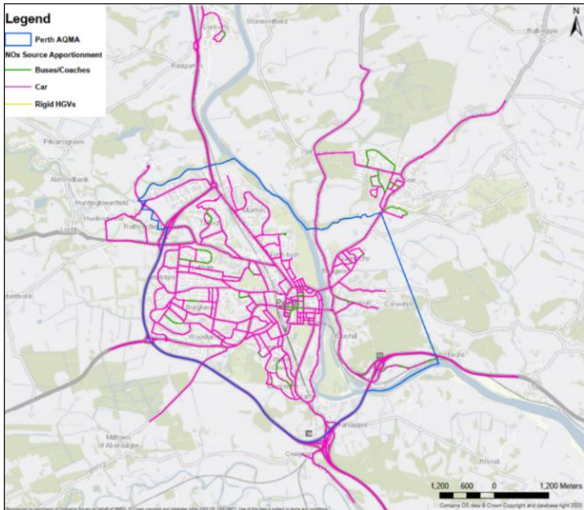
Figure 6.4: NO x Perth Source Apportionment Analysis
